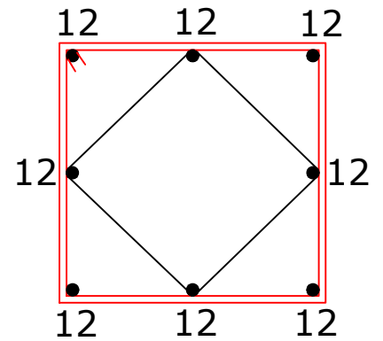
COLUMN - C1 SIZE 300mmX300mm
